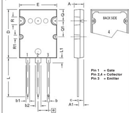
PLUS264™ (IXYB) Outline
