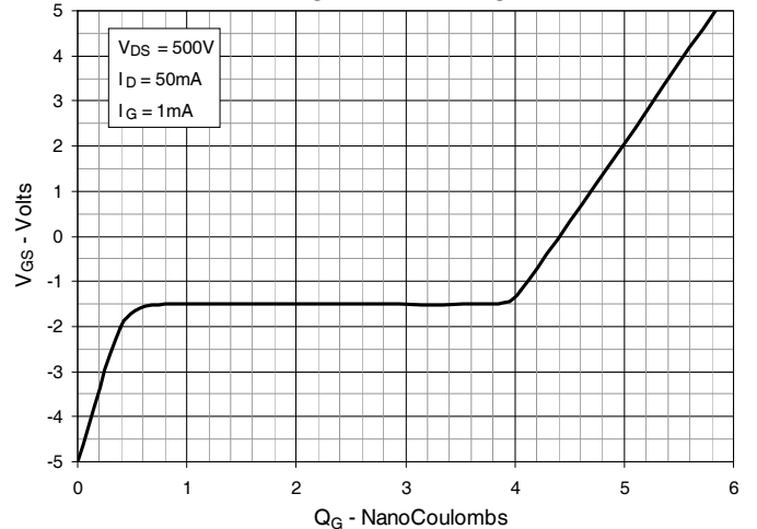
Fig. 12. Gate Charge
