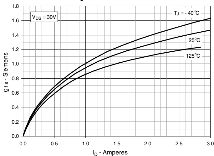
Fig. 10. Transconductance
