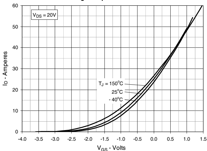
Fig. 9. Input Admittance
