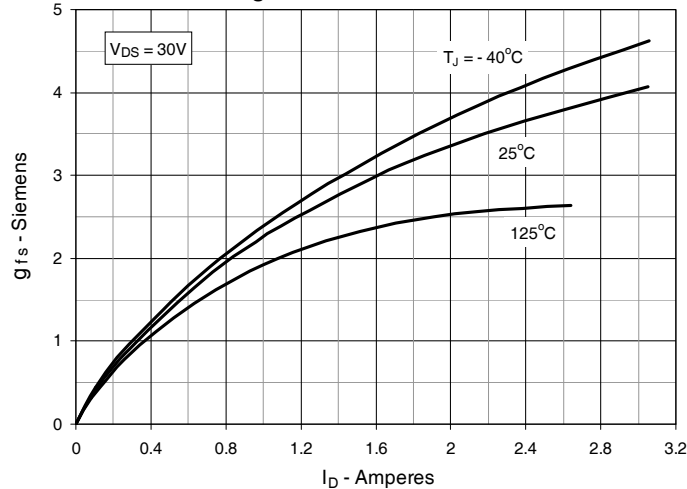
Fig. 11. Transconductance
