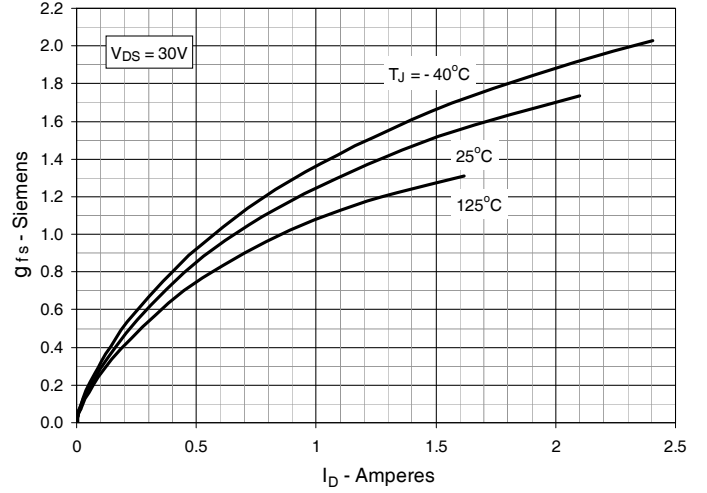
Fig. 10. Transconductance
