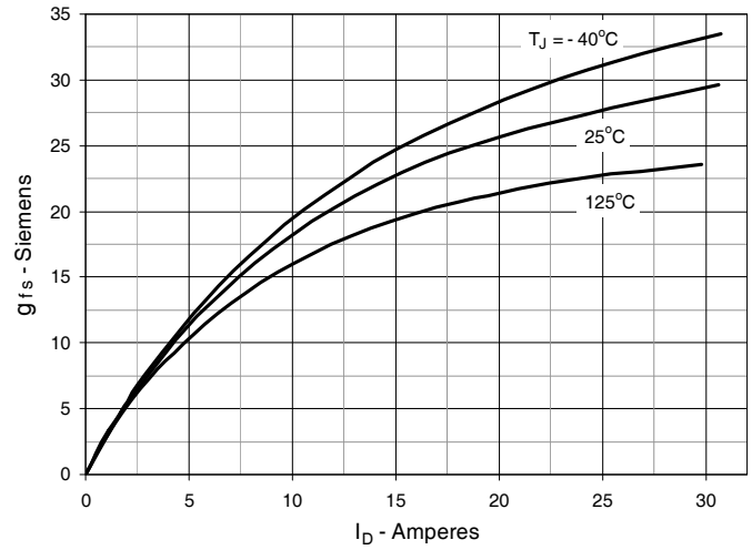
Fig. 8. Transconductance
