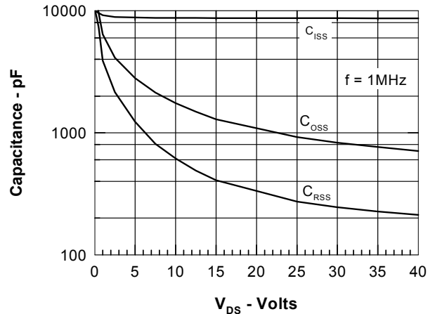
Figure 8. Capacitance Curves
