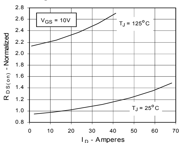
Fig. 5. R_{DS(on)} Normalized to I_D = 16\text{A} Value vs. Drain Current
