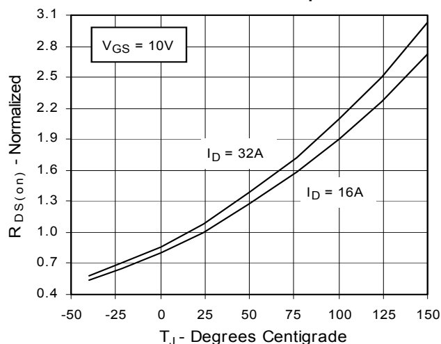
Fig. 4. R_{DS(on)} Normalized to I_D = 16\text{A} Value vs. Junction Temperature
