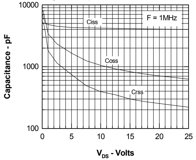
Figure 8. Capacitance Curves
