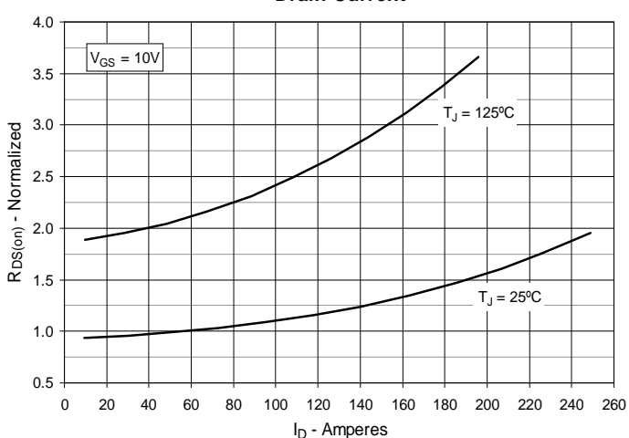
Fig. 5. R_{DS(on)} Normalized to I_D = 55\text{A} Value vs.
