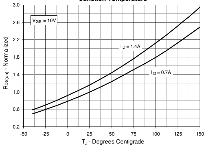
Fig. 4. R_{DS(on)} Normalized to I_D = 0.7A Value vs. Junction Temperature
