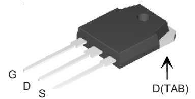
TO-3P (IXTQ)
