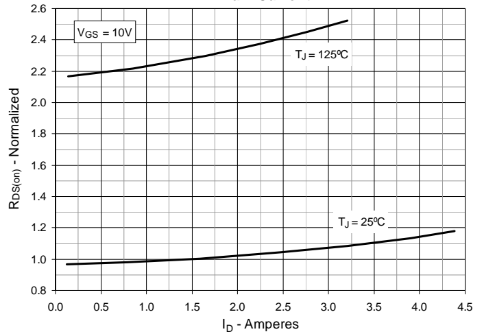
Fig. 4. R_{DS(on)} Normalized to I_D = 1.5A Value vs. Drain Current
