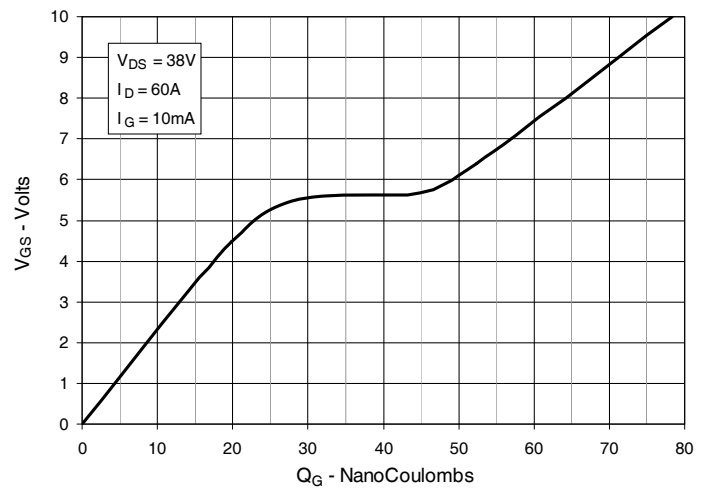
Fig. 10. Gate Charge
