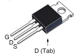
TO-220 (IXTP)
