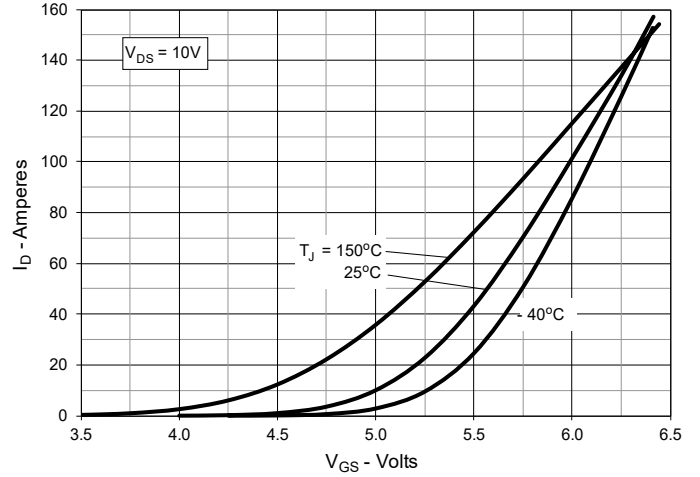
Fig. 8. Input Admittance
