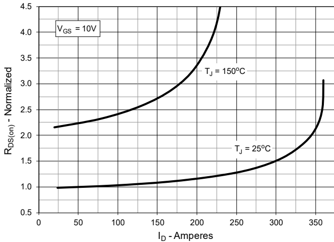
Fig. 5. R_{DS(on)} Normalized to I_D = 47A Value vs. Drain Current
