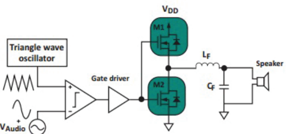
Figure 3: Half-bridge Class-D audio amplifier
