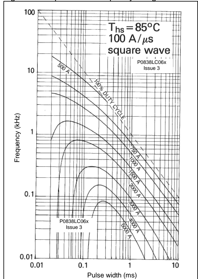
Figure 11 - Square wave frequency ratings
