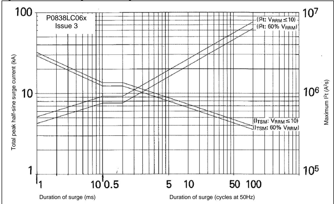
Figure 16 - Maximum surge and I 2 t Ratings at initial T J – 125°C
