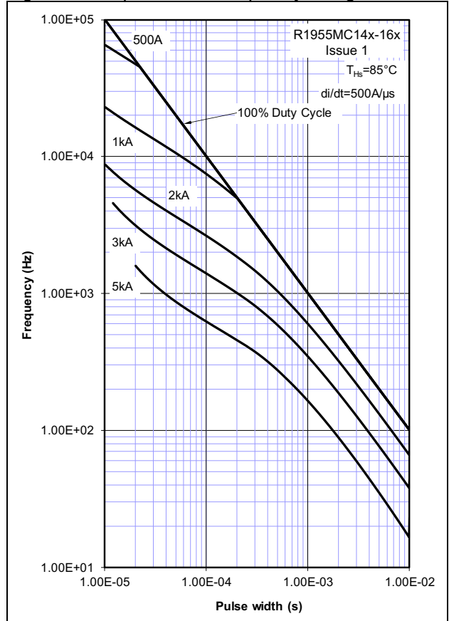
Figure 16 - Square wave frequency ratings
