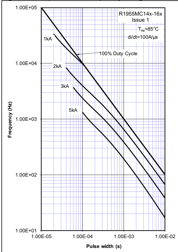
Figure 15 - Square wave frequency ratings
