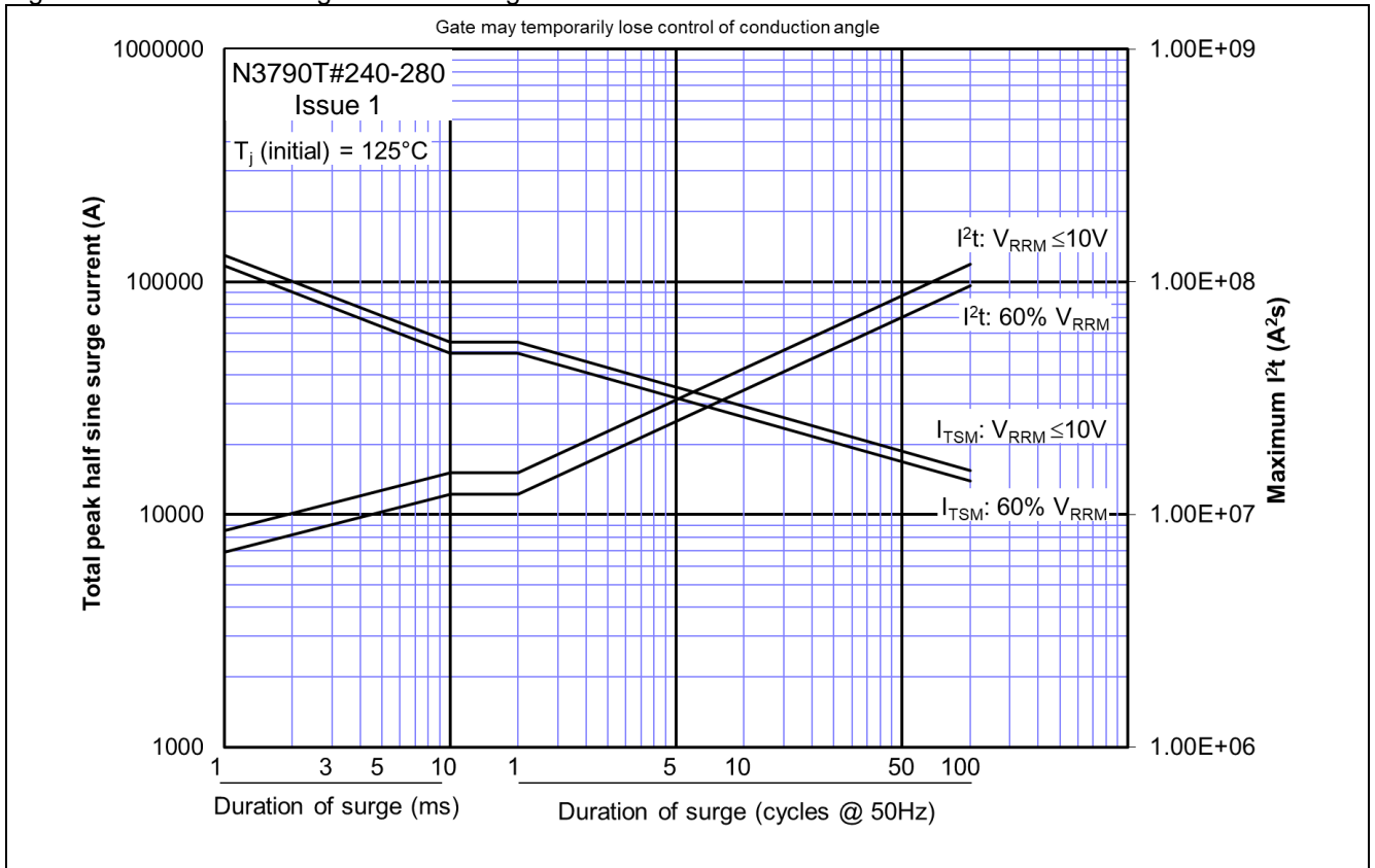
Figure 16 – Maximum surge and I^2t Ratings
