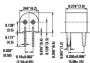
Circuit Board Mounting Detail
