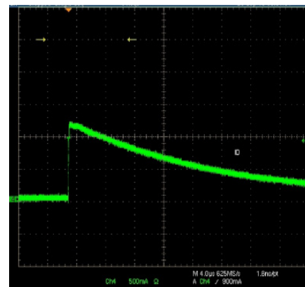
Figure 5. Bootstrap inrush current with RBS=10Ω, CBS=2.2μF
