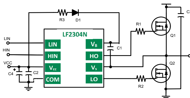
Figure 13. Schematic for layout example shown in figure 14.
