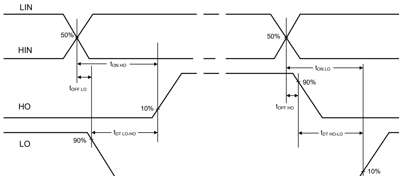
Figure 2. Input-to-Output Delay Timing Diagram
