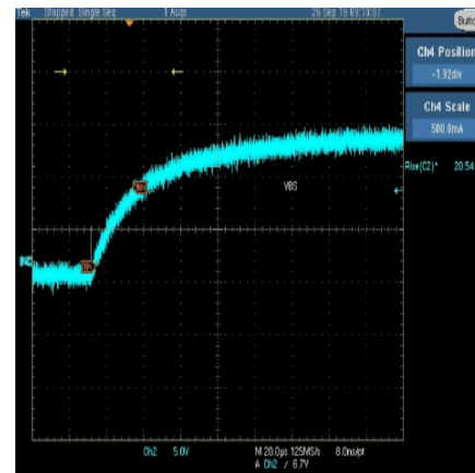
Figure 7. VBS rise time (20.5μs) with CBS=2.2μF and RBS=10Ω resistor
