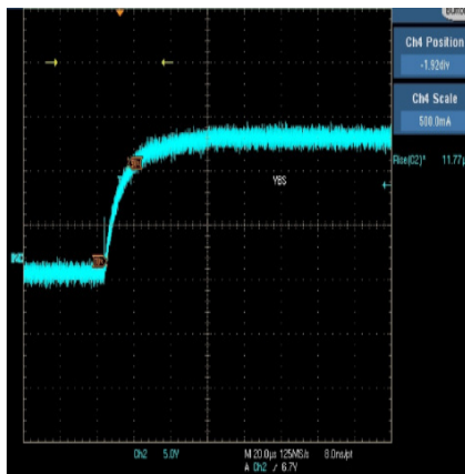
Figure 6. VBS rise time (11.8μs) with CBS=2.2μF and RBS=3Ω resistor
