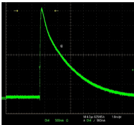
Figure 4. Bootstrap inrush current with RBS=3Ω, CBS=2.2μF
