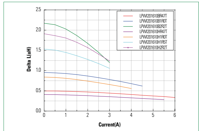
Inductive Vs. DC Current Characteristics 2.0 x 1.2 x 0.8 mm size
