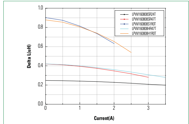
Inductive Vs. DC Current Characteristics 1.6 x 0.8 x 0.8 mm size
