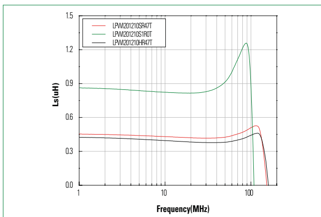
Inductive Vs. Frequency Characteristics 2.0 x 1.2 x 1.0 mm size
