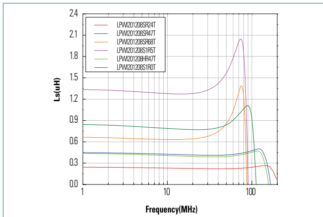
Inductive Vs. Frequency Characteristics 2.0 x 1.2 x 0.8 mm size
