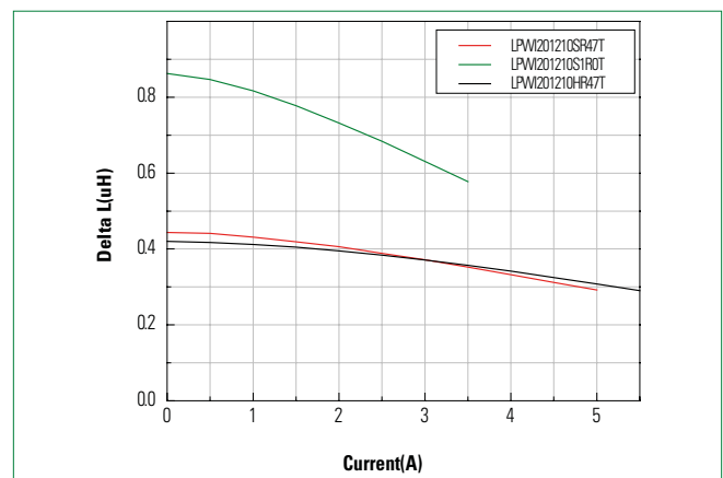
Inductive Vs. DC Current Characteristics 2.0 x 1.2 x 1.0 mm size
