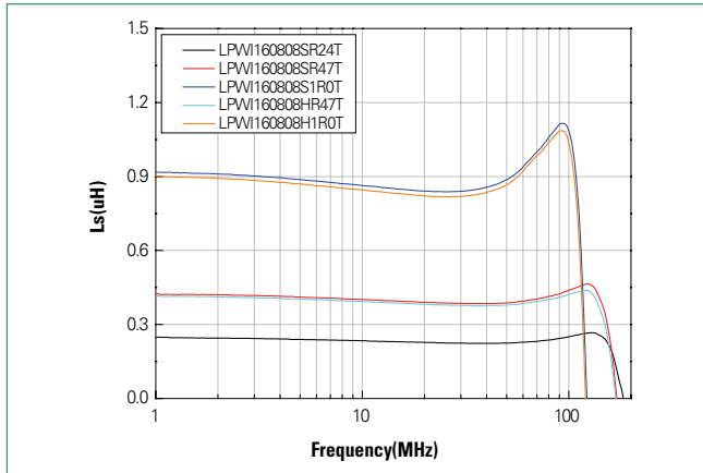
Inductive Vs. Frequency Characteristics 1.6 x 0.8 x 0.8 mm size
