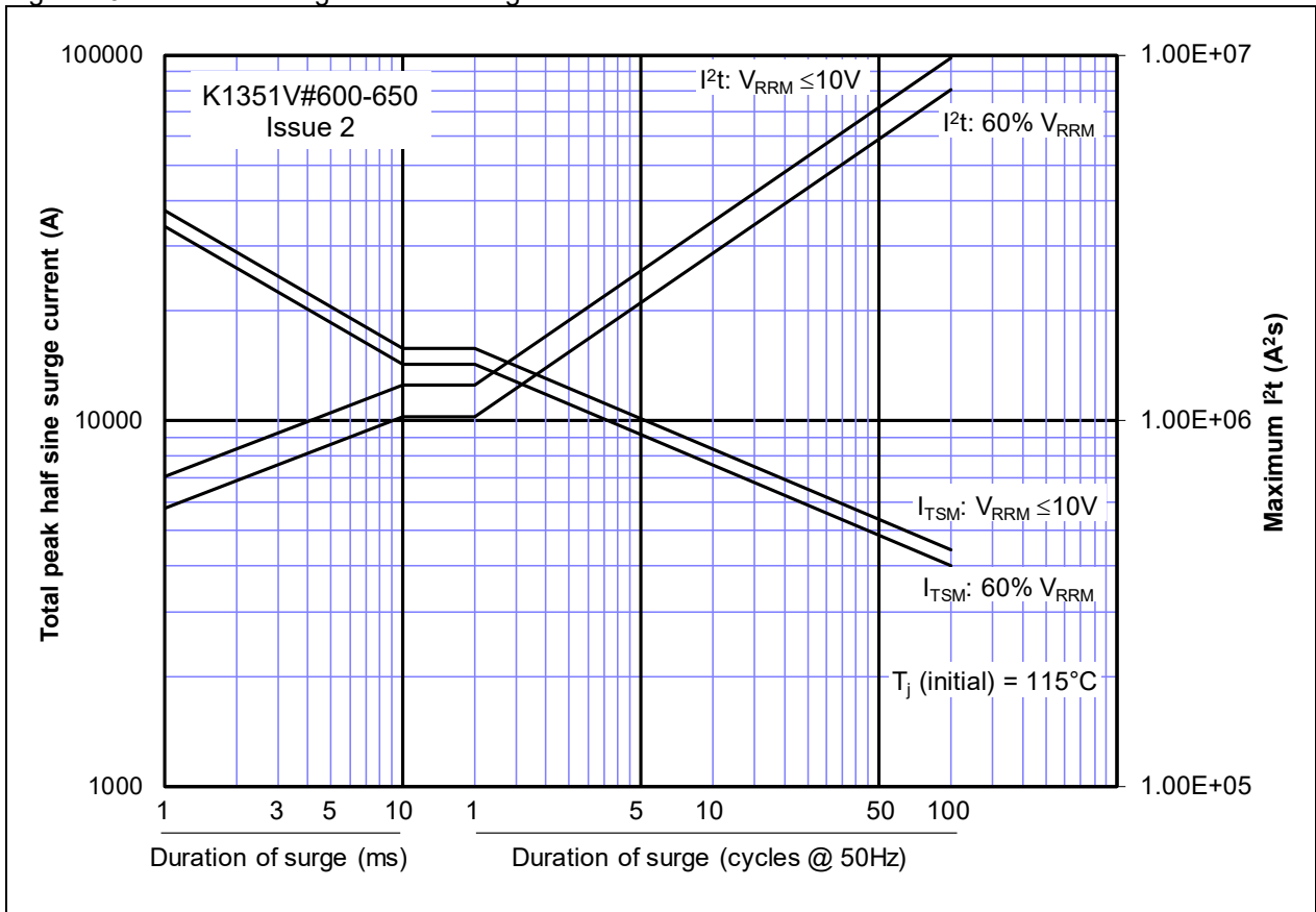
Figure 19 - Maximum surge and I²t Ratings
