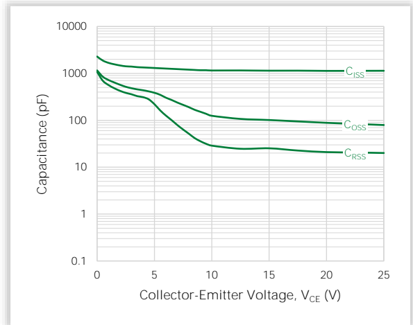
Figure 10. Capacitance Variance
