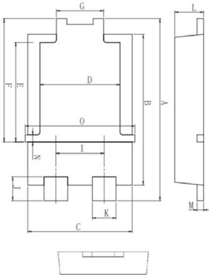
Dimensions-TO-277B
