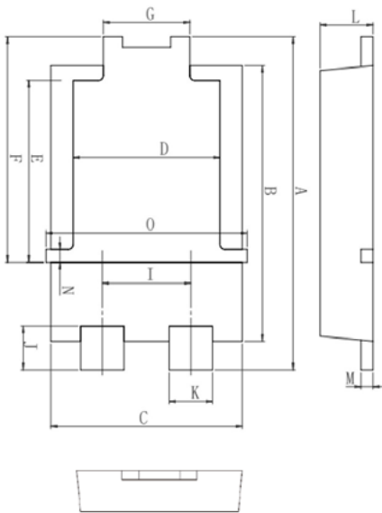
Dimensions-TO-277B
