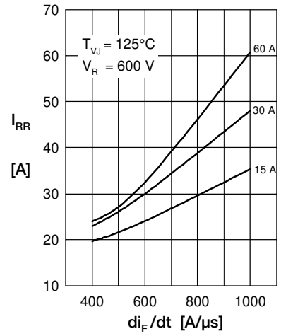
Fig. 3 Typ. peak reverse current I_{RRM} versus di/dt
