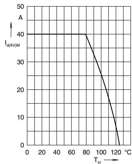
Fig. 7 Max. forward current vs. heatsink temperature
