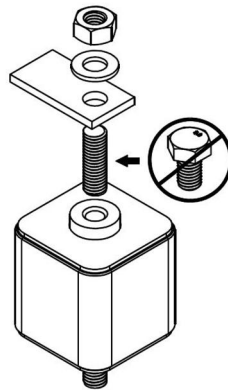
Figure 40: Recommended means for fuse termination
