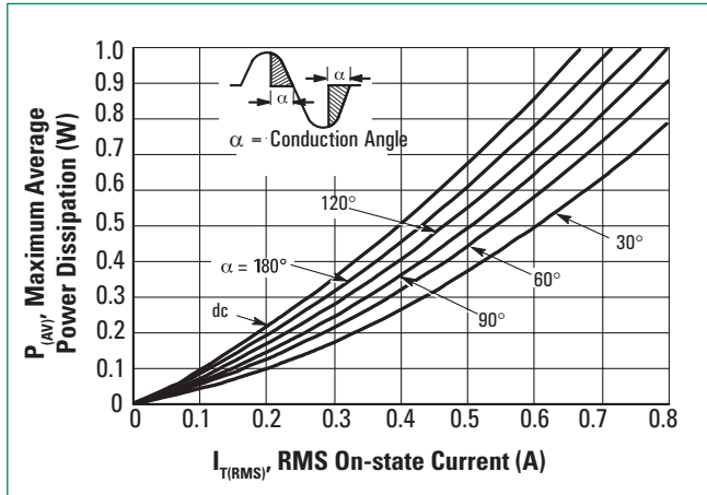
Figure 8. Power Dissipation
