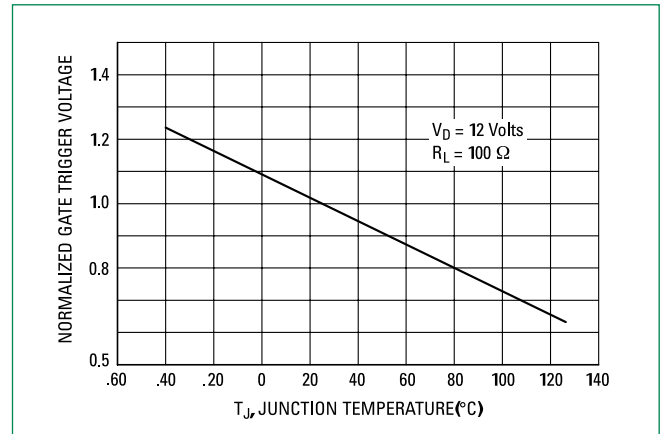
Figure 7. Gate Trigger Voltage
