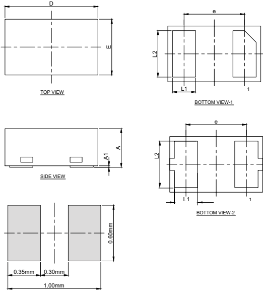
Recommended Soldering Pattern
