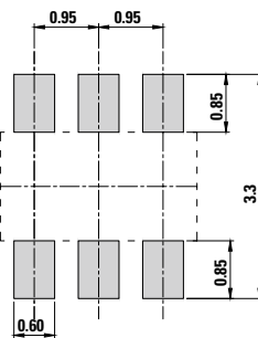
Recommended soldering pad layout (unit :mm)
