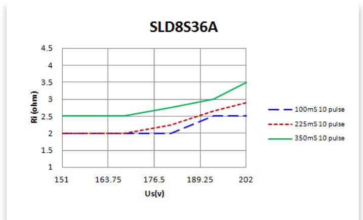
Figure 19. 24v system 10pulses(ISO16750-2) U_s Vs. R_i
