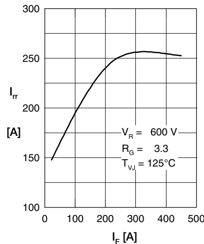
Fig. 5 Typ. reverse recovery characteristics
