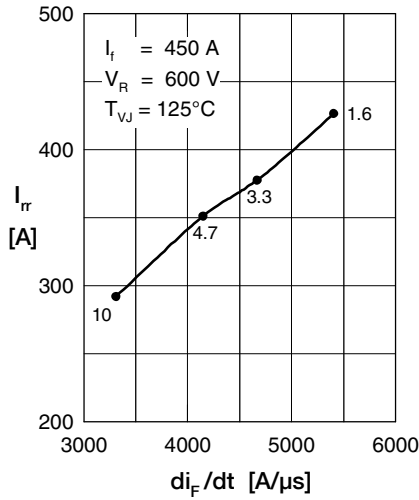
Fig. 2 Typ. reverse recovery characteristics
