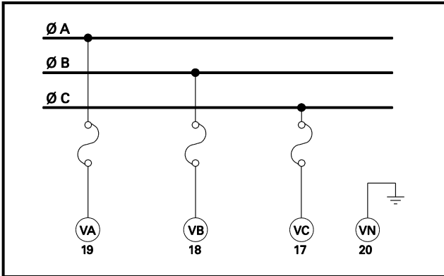
FIGURE 3.3 Direct Connection.
