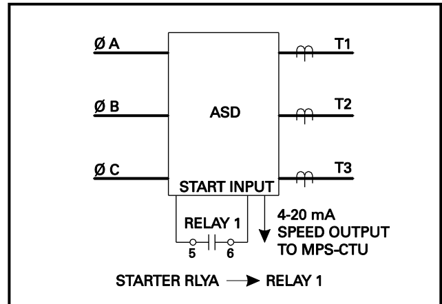
FIGURE 6.10 Adjustable-Speed-Drive Connection.
