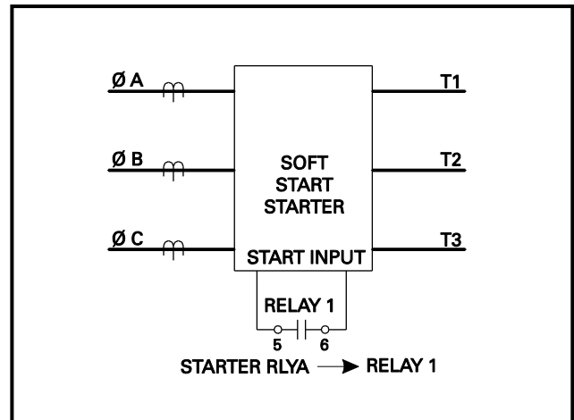
FIGURE 6.11 Soft-Start-Starter Connection.
