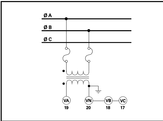
FIGURE 3.4 1-PT Connection.
