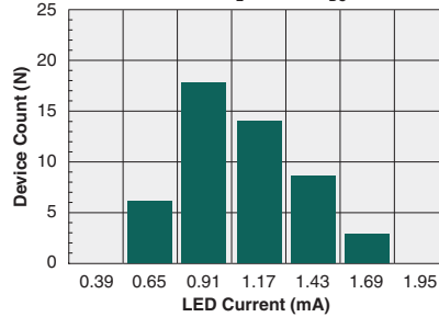
Typical I F for Switch Dropout (N=50, I L =120mA DC )
