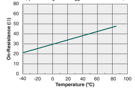
Typical On-Resistance vs. Temperature ( I_F=5\text{mA} , I_L=50\text{mA}_{DC} Instantaneous)
