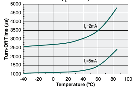
Turn-Off Time vs. Temperature (I L =75mA)
