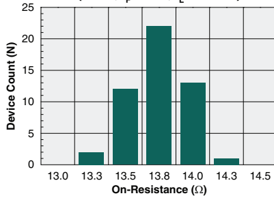
Typical On-Resistance Distribution (N=50, I F =0mA, I L =100mA)
