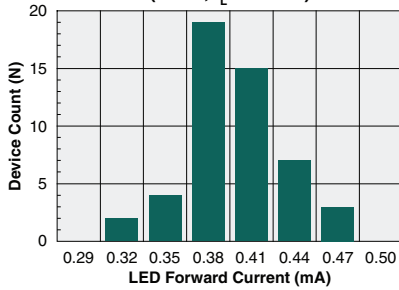
Typical LED Forward Current to Activate (N=50, I L =100mA)
