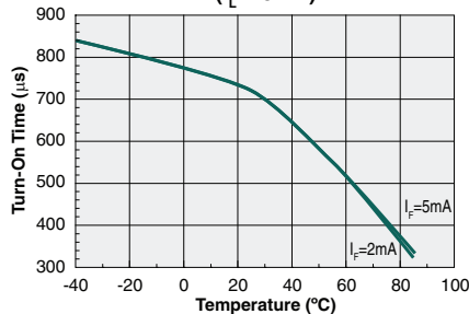
Turn-On Time vs. Temperature (I L =75mA)
