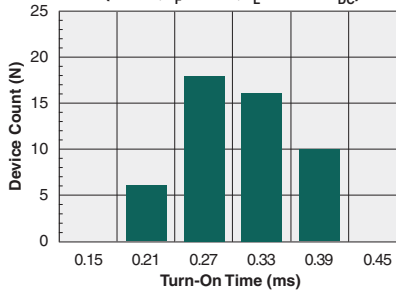
Typical Turn-On Time (N=50, I_F=5mA , I_L=150mA_{DC} )
