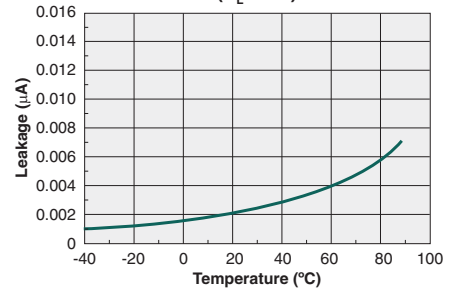
Typical Leakage vs. Temperature Measured Across Pins 4&6 ( V_L=60\text{V} )
