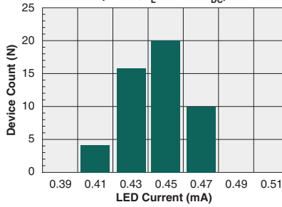
Typical I_F for Switch Dropout (N=50, I_L=600mA_{DC} )
