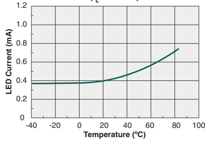
Typical I_F for Switch Dropout vs. Temperature ( I_L=300\text{mA} )
