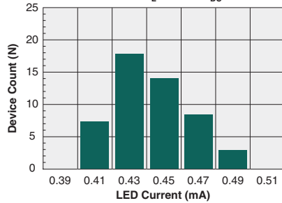
Typical I_F for Switch Operation (N=50, I_L=600mA_{DC} )
