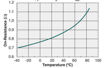
Typical On-Resistance vs. Temperature ( I_F=2\text{mA} , I_L=600\text{mA}_{DC} )
