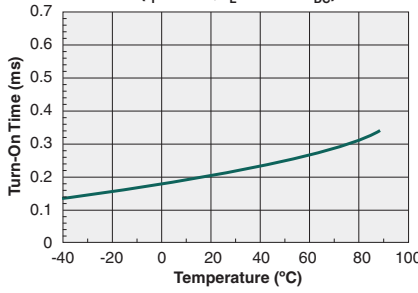
Typical Turn-On Time vs. Temperature ( I_F=5\text{mA} , I_L=200\text{mA}_{DC} )
