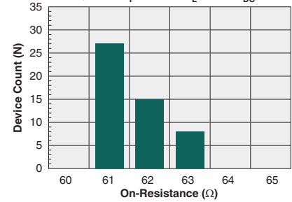
Typical On-Resistance Distribution (N=50, I_F=10\text{mA} , I_L=50\text{mA}_{DC} )
