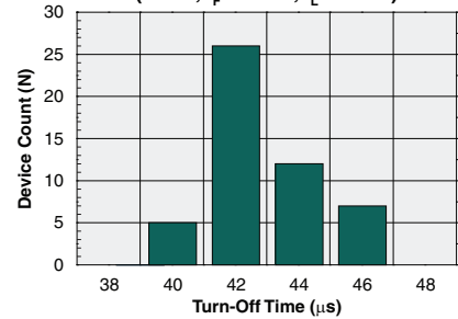
Turn-Off Time Distribution (N=50, I_F=10\text{mA} , I_L=50\text{mA} )
