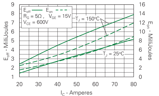
Fig. 12. Inductive Switching Energy Loss vs. Collector Current
