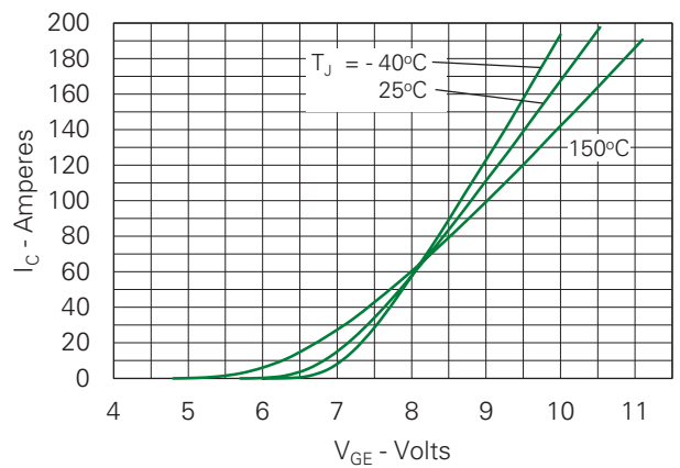
Fig. 6. Input Admittance
