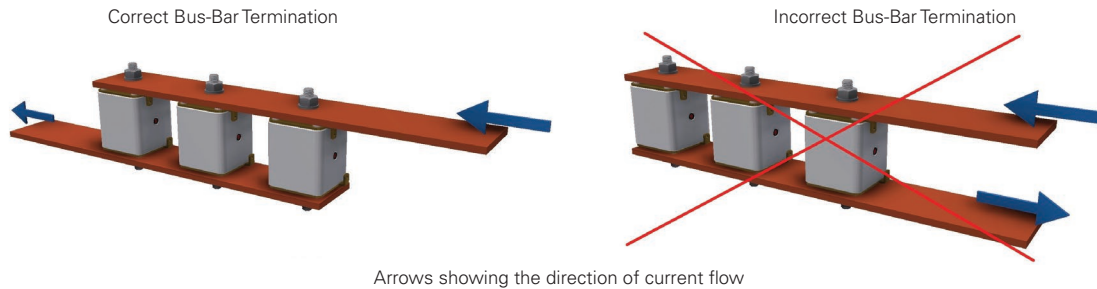
Figure 37. Paralleling two or more high-speed fuses
