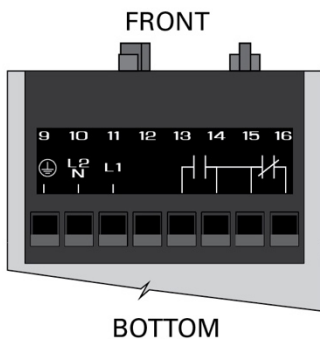
FIGURE 1A. SE-703-0X-00 Outline and Mounting Details.
